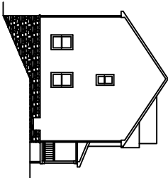
LEFT ELEVATION
